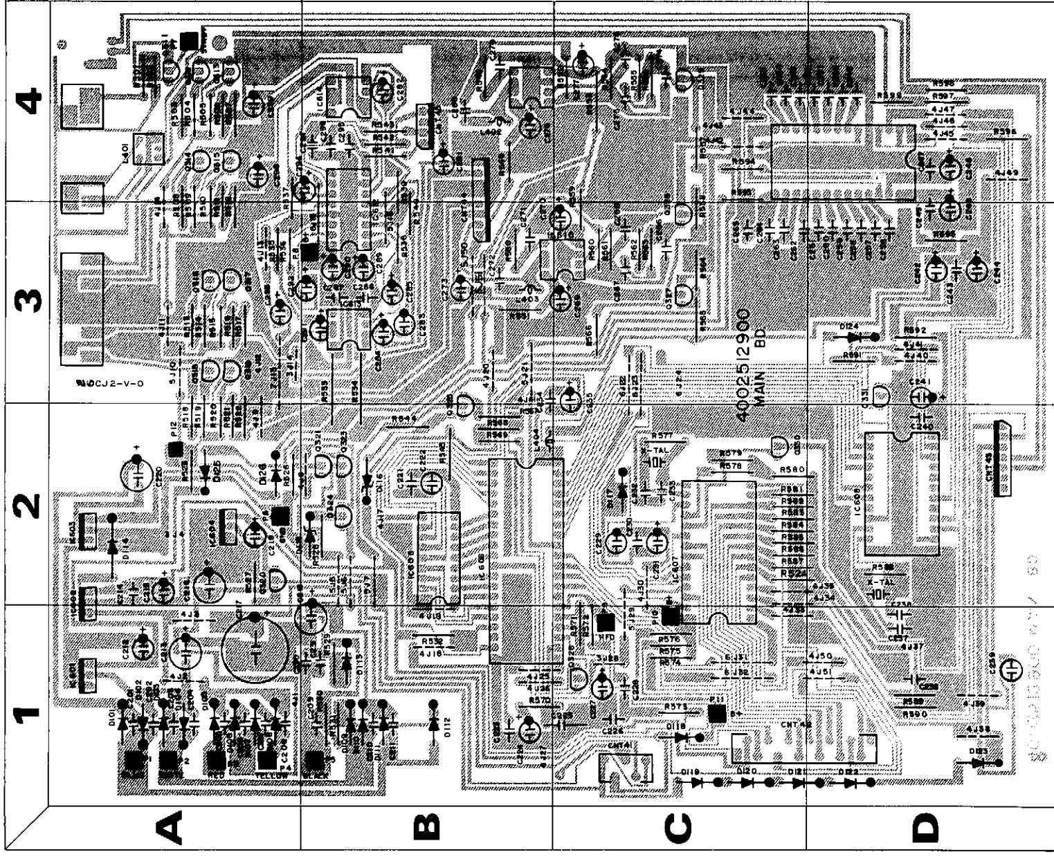
MAIN BOARD 4002512900
