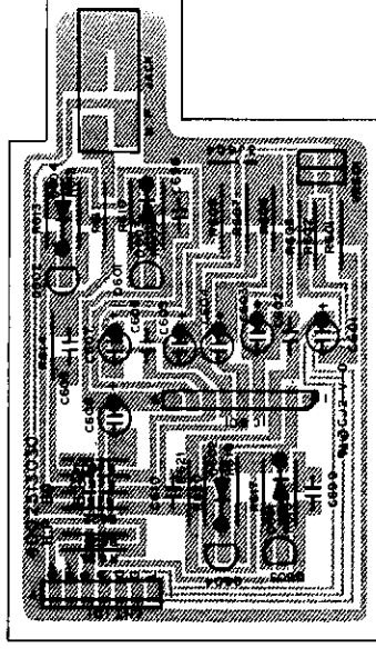
H.P. BOARD 4002513030
