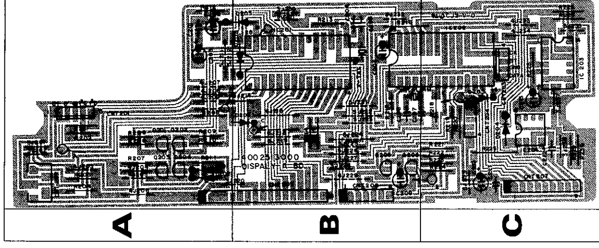
DISPLAY BOARD-A 4002513000
